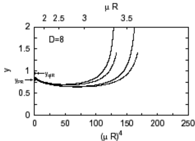
FIG. 10: RGE flows for the top Yukawa coupling y . We also show the quasi IR fixed point y_{qIR} and the PR fixed point y_{PR} at \mu = R^{-1} . The graph represents running of y for D = 8 . R^{-1} = 10 \text{ TeV} was assumed. We used the full one-loop RGE (51). The UV-BCs are y(\Lambda) \rightarrow \infty (solid lines) and y(\Lambda) = \sqrt{2} (dashed and dash-dotted lines) for two typical values of \Lambda .
